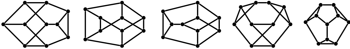
FIGURE 5. The graphs appearing in the unique nonzero reduced homology class in \Delta_6 , with unsigned coefficients 2, 3, 6, 3, 4.
