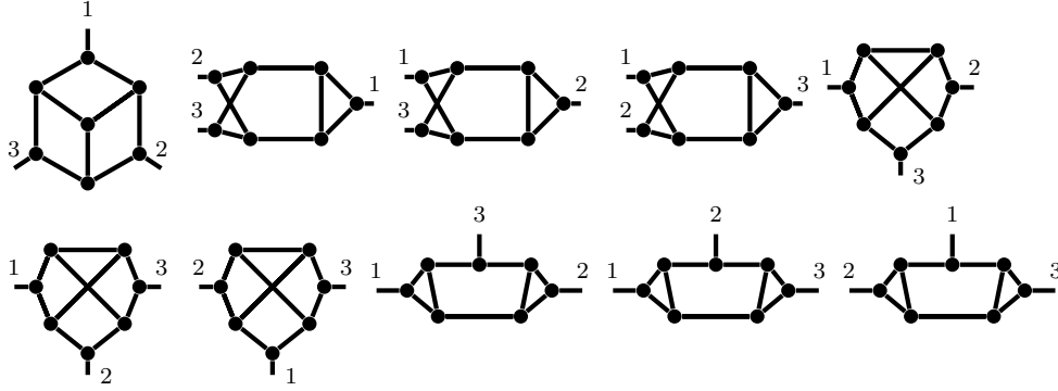
FIGURE 4. The graphs appearing in the unique nonzero reduced homology class in \Delta_{3,3} , with unsigned coefficients 1, 1, 1, 1, 1, 1, 1, 2, 2, 2.
