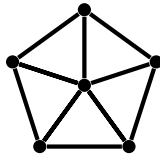
FIGURE 3. The graph W_5 .
