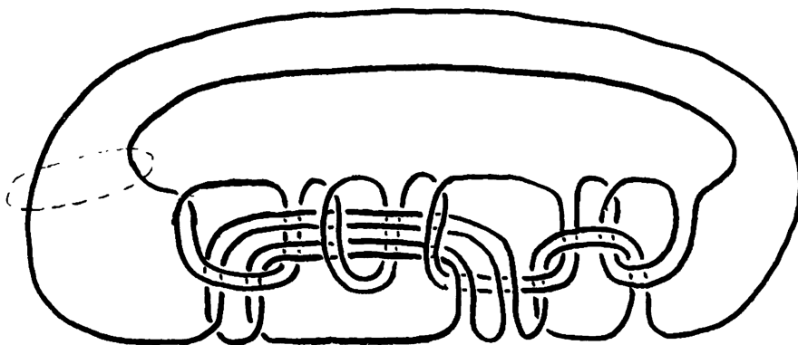
downstairs branch set in branched covering M^3 \rightarrow S^3
