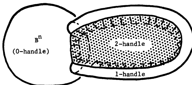
A 2-handle cancelling a 1-handle
