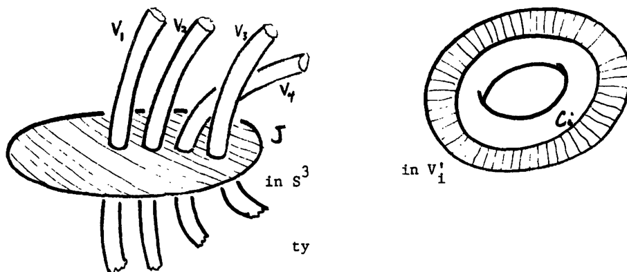
typical fibre (shaded)
