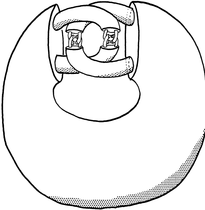
ALEXANDER'S HORNED SPHERE
