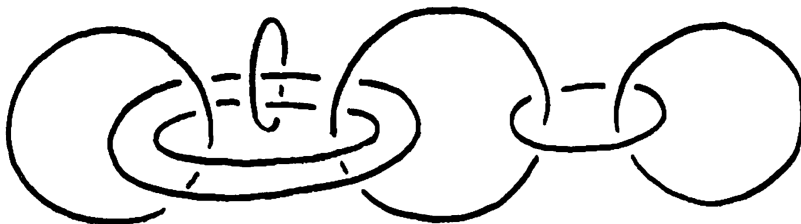
typical surgery curves in S^3
