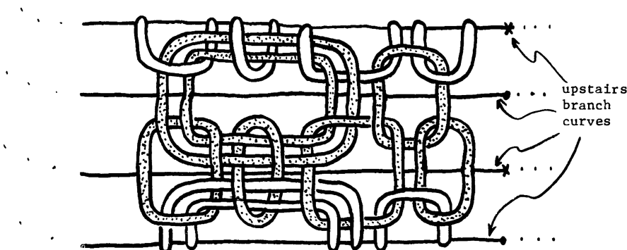
in the upstairs S^3
