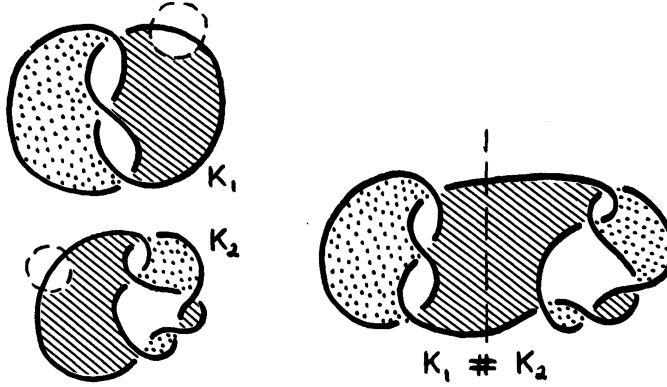
boundary connected sum of two surfaces makes a Seifert surface for K_1 \# K_2 .
