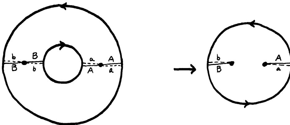
2-fold branched cover of D^2 by S^1 \times I
