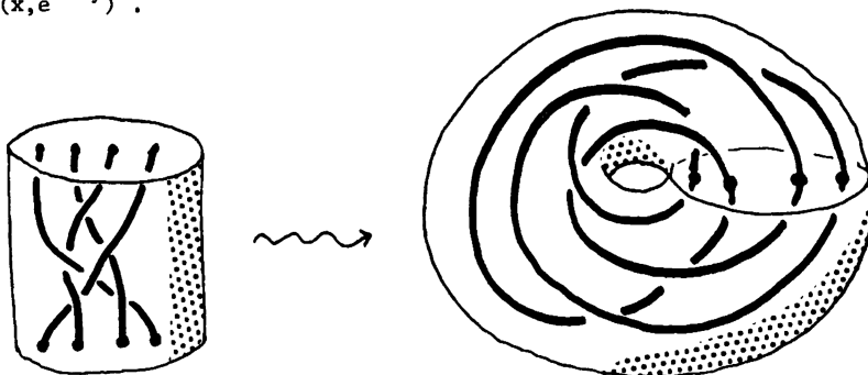
A braided link in a solid torus
