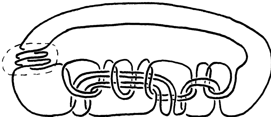
revised branch set which is connected
