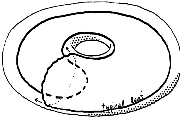
Reeb foliation of the solid torus.
