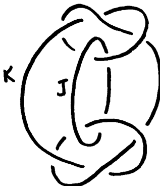
The Andrews-Curtis link C \cup D spun by S^0
