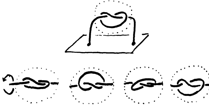
a full twist of the knot in R_+^3
