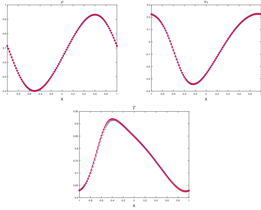
Figure 7: Test II (a). ‘DS’ (circle) versus ‘MM’ (asteroid). \varepsilon = 1 , t = 0.25 .
