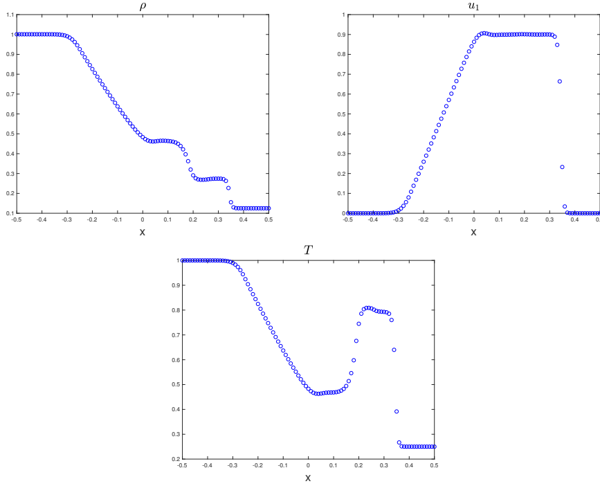
Figure 8: Test II (b). Numerical solutions by ‘MM’. \varepsilon = 10^{-3} , t = 0.2 .
