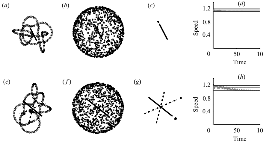
FIGURE 4. Sedimentation simulations for filaments in the shapes of ideal 7_7 ( a – d ) and 7_1 knots ( e – h ). ( a ) The hydrodynamic axis of the ideal 7_7 knot defined by the single real eigenvector \pm\eta_{\text{real}} of M_2 . ( e ) The three hydrodynamic axes of the ideal 7_1 knot defined by the eigenvectors \pm\eta_{\text{min}} (dot-dashed), \pm\eta_{\text{mid}} (dashed) and \pm\eta_{\text{max}} (solid) of M_2 . ( b ), ( f ) Distribution of gravity directions in the body frame of each knot at t=0 . ( c ), ( g ) Distribution of gravity directions in the body frame of each knot at t=200 . The simulations were performed with the exact equations of motion (3.3) with \varepsilon=0.01 . ( d ), ( h ) Time histories of sedimentation speed \vartheta for various members of the sample for each knot. The two horizontal lines in each plot correspond to the eigenvalues \theta_{\text{min}} and \theta_{\text{max}} of M_1 for each knot. (The time histories in panel ( d ) are partially obscured by the lower horizontal line).
