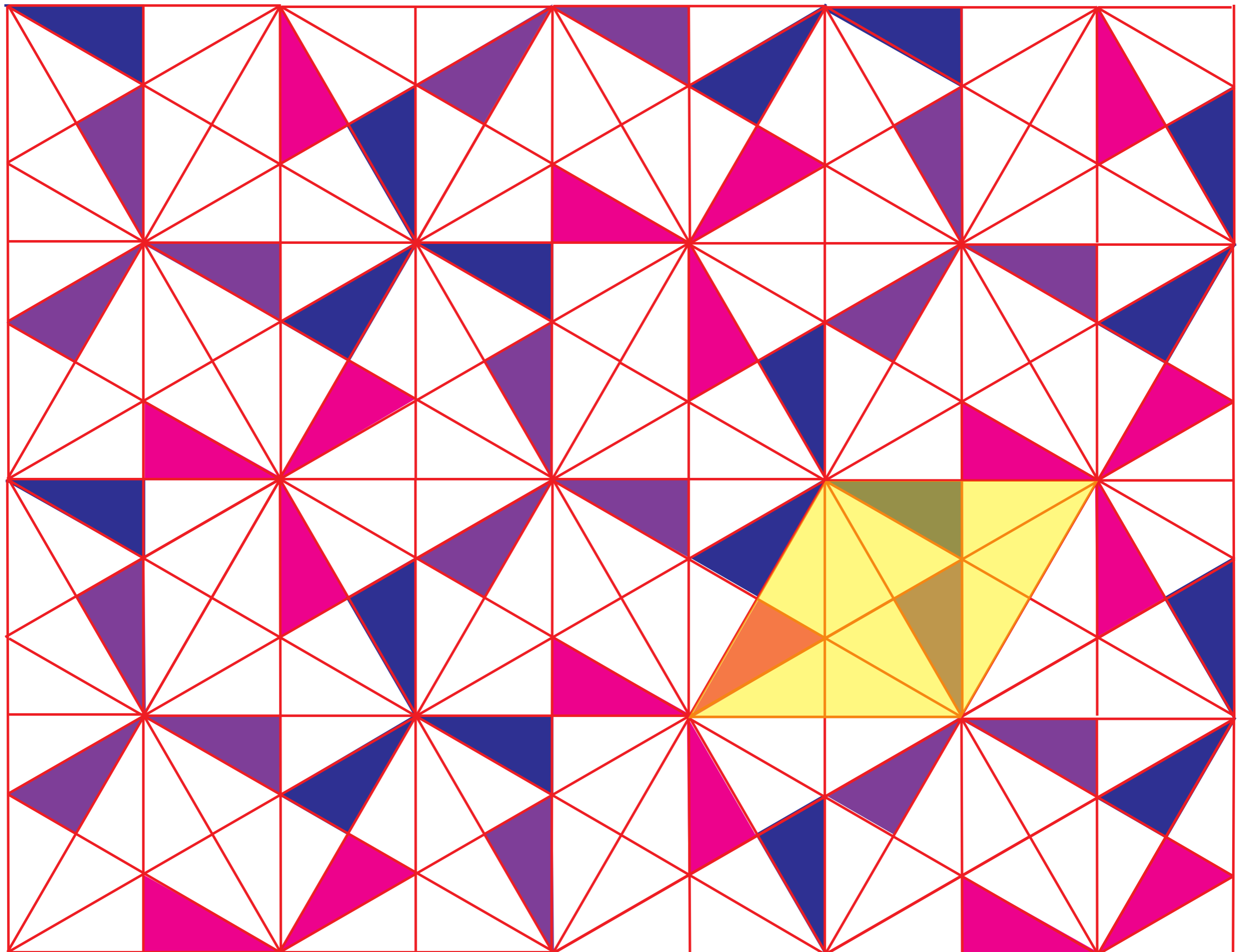
The yellow parallelogram (including two of its edges) is a fundamental domain.
