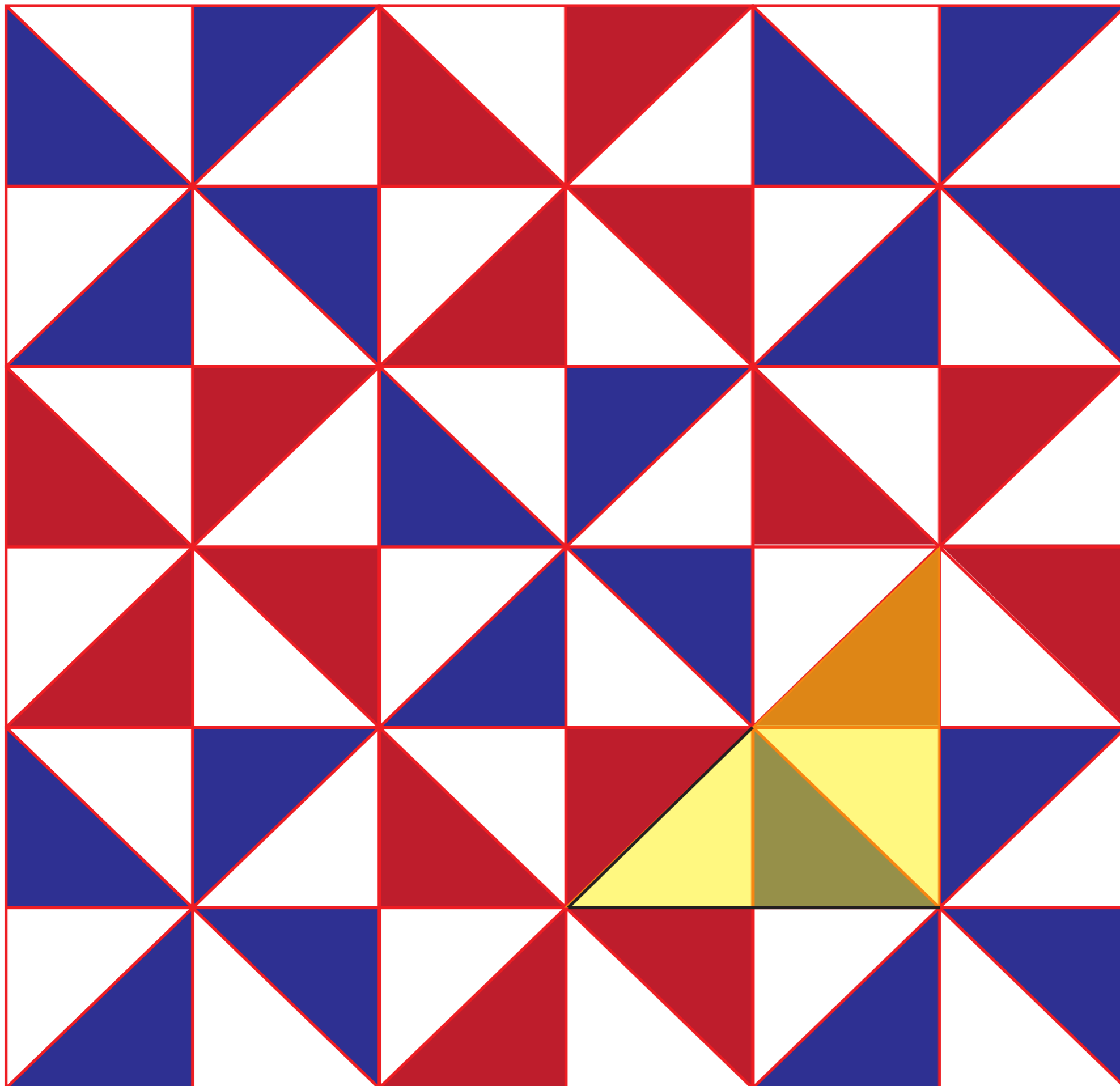
The yellow/orange/brown triangle, including the black parts of its boundary, is a fundamental domain.
