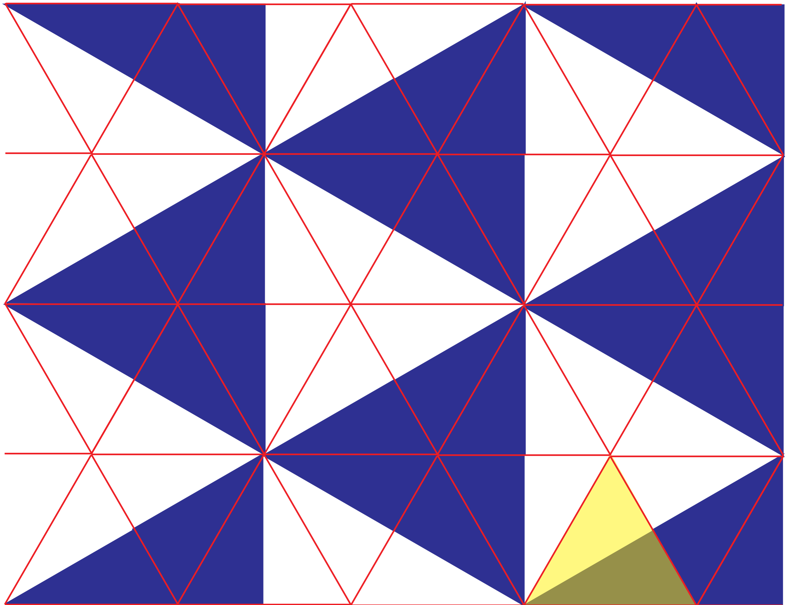
The yellow/brown equilateral triangle, including its boundary, is a fundamental domain. It is also the orbifold for this pattern.
