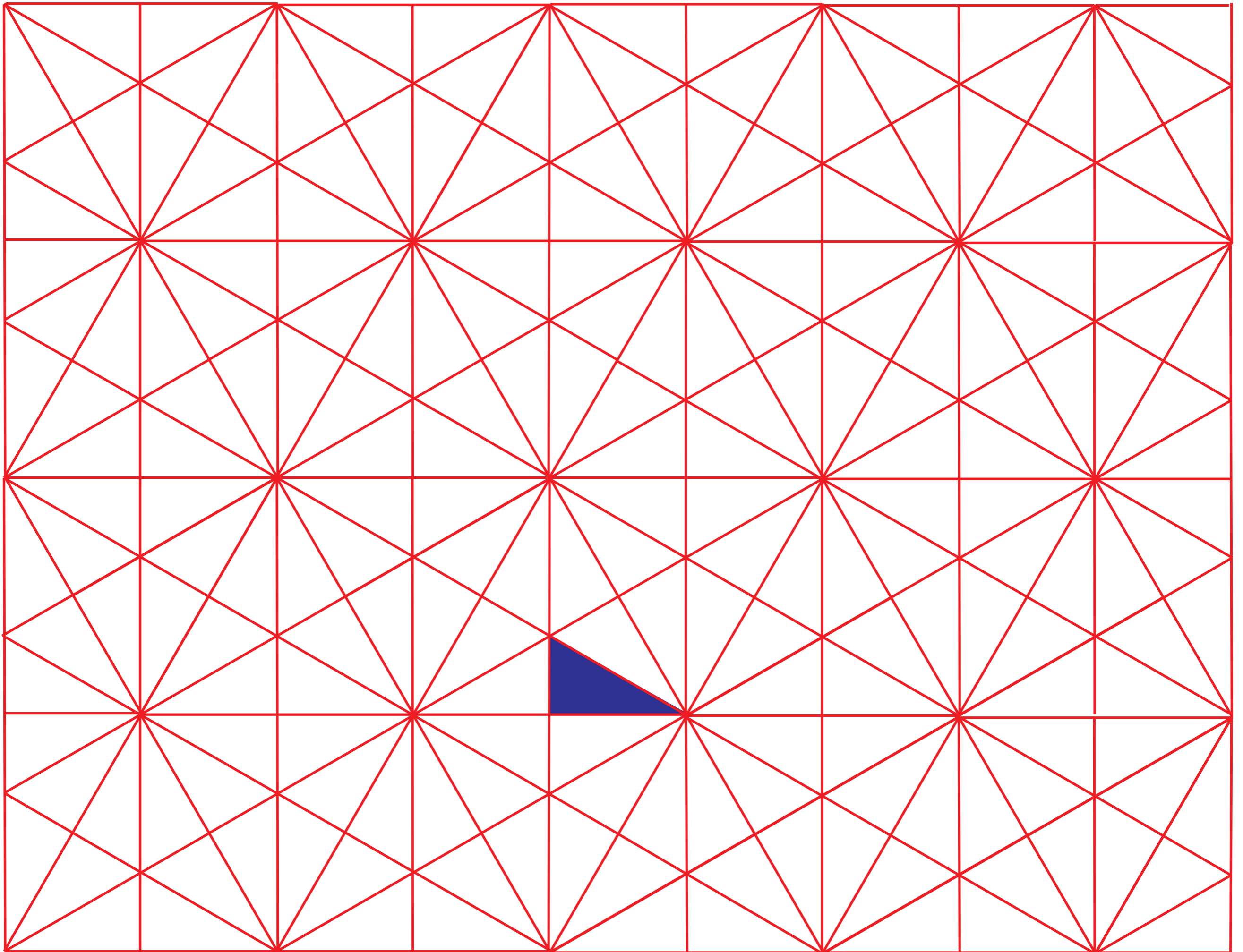
The blue triangle (including its boundary) is a fundamental domain. It is also the orbifold for this pattern.
