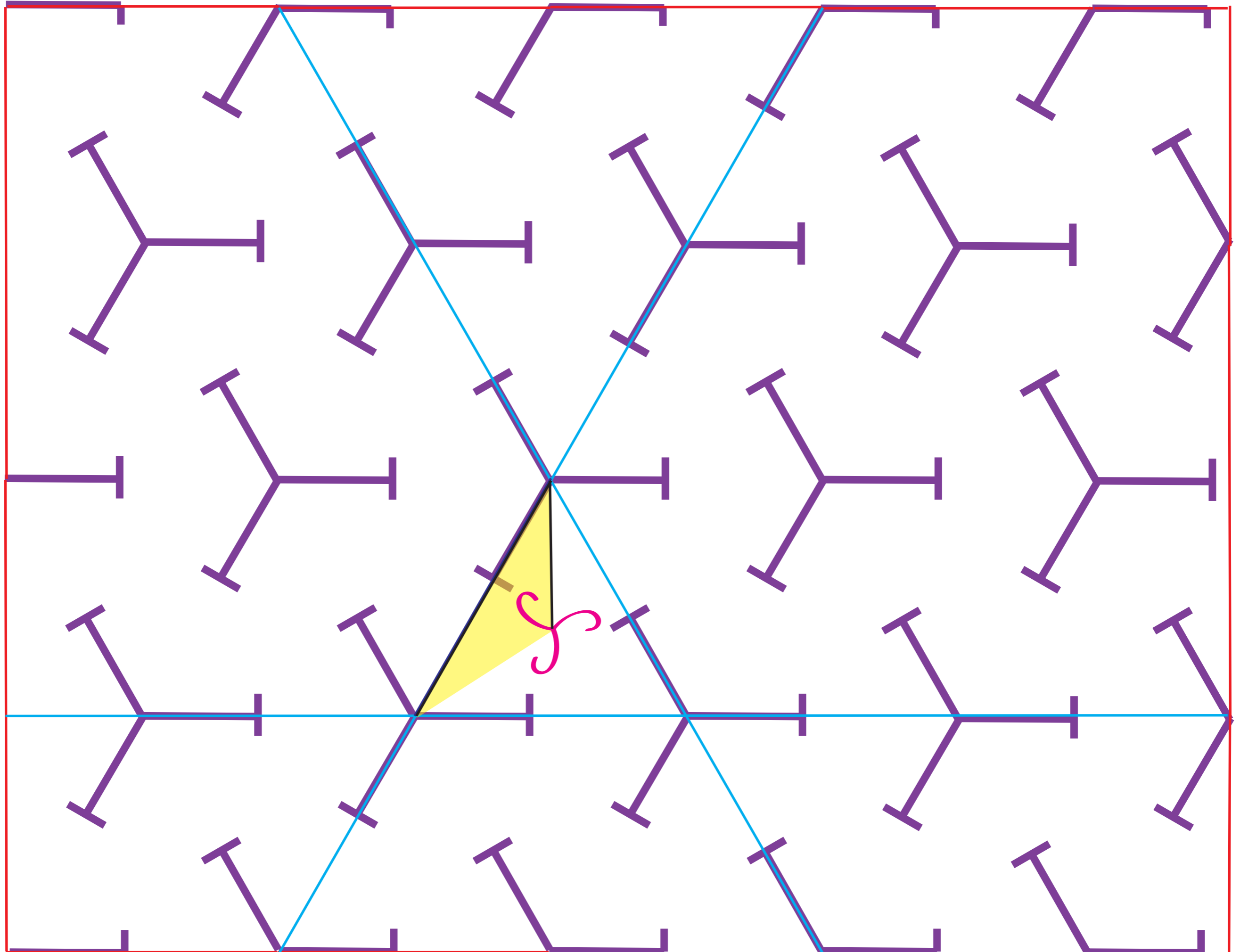
Three equivalent mirrors and a rotation center are shown. The yellow triangle, including its two black edges, is a fundamental domain.
