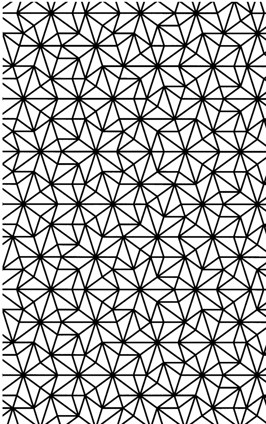
Figure 4. A Penrose tiling.
