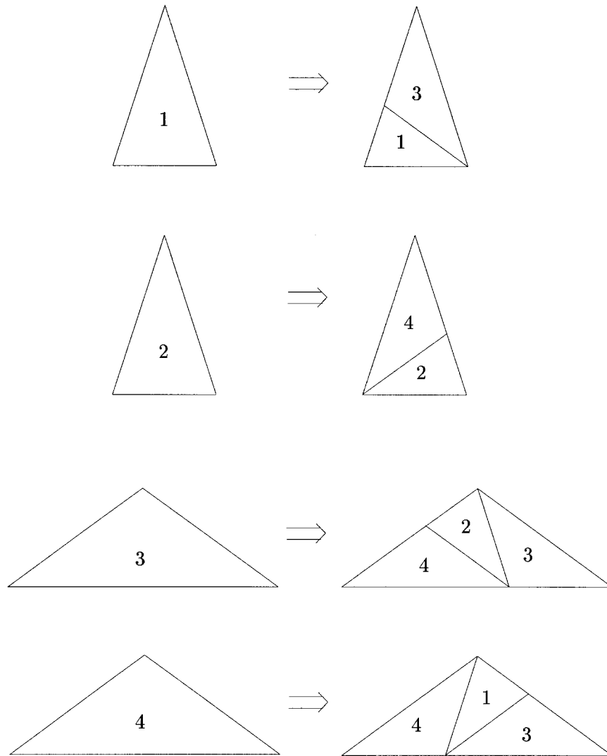
Figure 5. The Penrose substitution.
