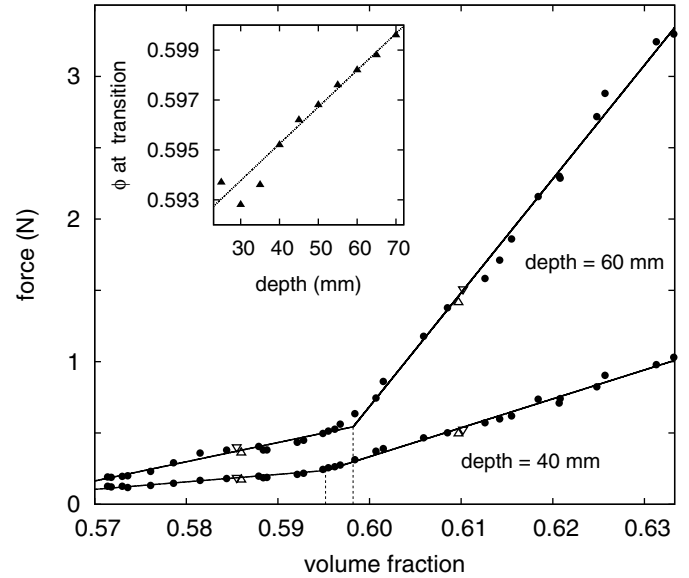
Fig. 2: The dependence of the penetration force on volume fraction changes at \phi = 0.598 at a depth of 60 mm. Data represented by \bullet were measured at a penetration speed of 10 mm/min, \nabla at 5 mm/min and \Delta at 20 mm/min. The transition points were determined by the intersection of least-square fits for the volume fractions below and above the intersection, excluding points near the transition. The inset displays the dependence of the transition point on the penetration depth.
