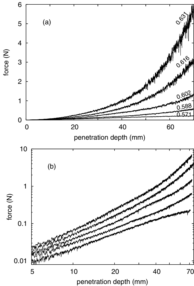
Fig. 1: (a) Penetration force as a function of depth for different volume fractions. (b) Log-log plot of the data in (a). These curves are measured with a penetration speed of 10 mm/s, but the results are the same for a range of penetration speeds. The total sample height is 110 mm (at \phi = 0.6 ).
