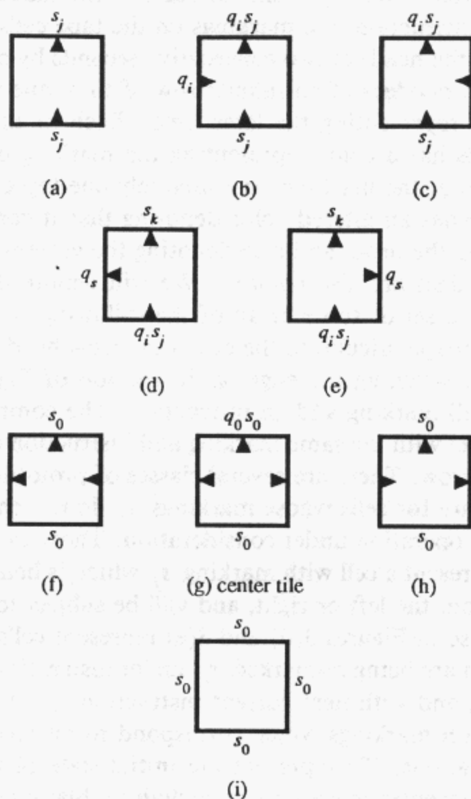
FIGURE 3. Prototiles used to mirror a Turing machine.
