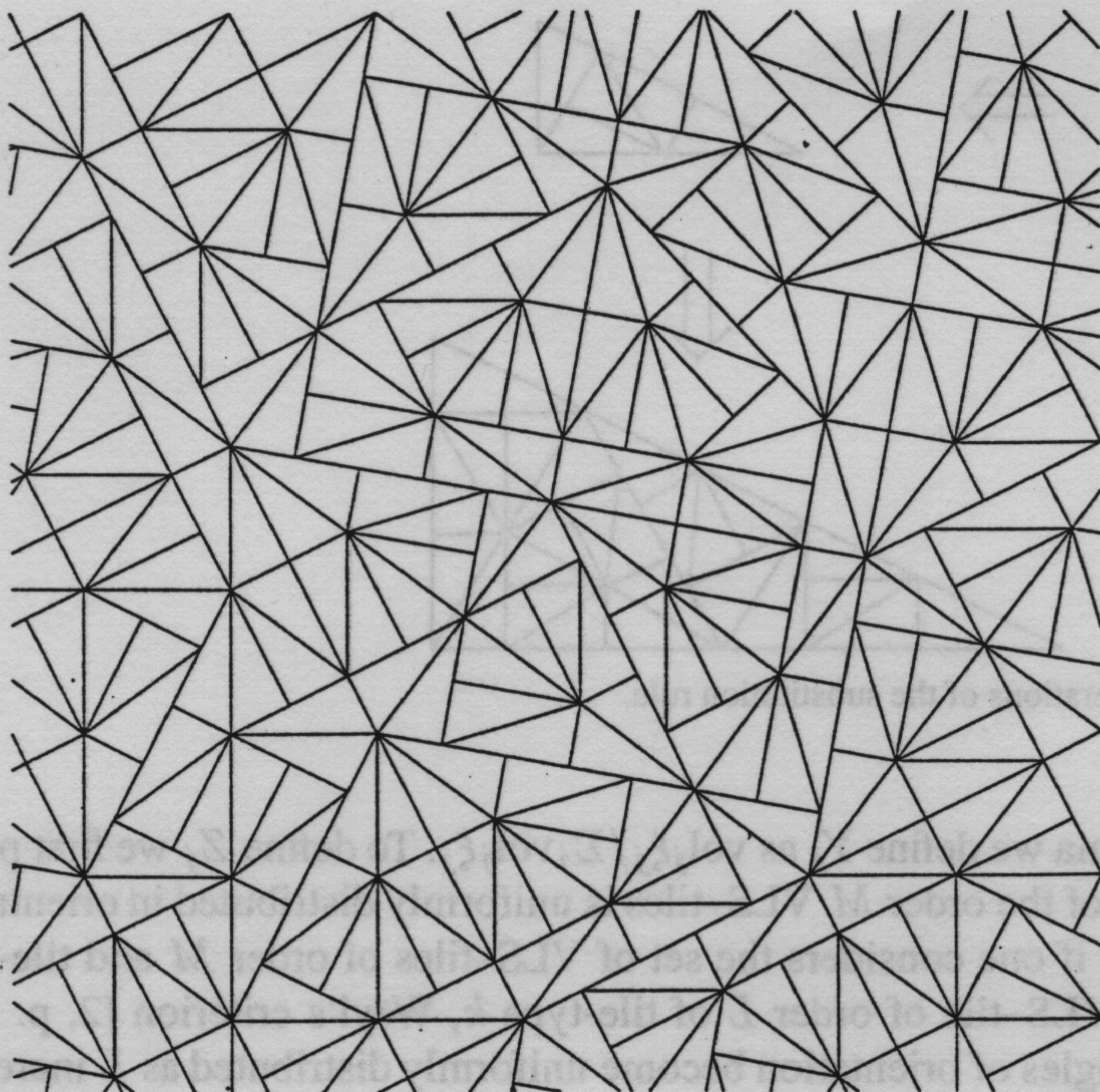
Fig. 2. Part of a pinwheel tiling.
