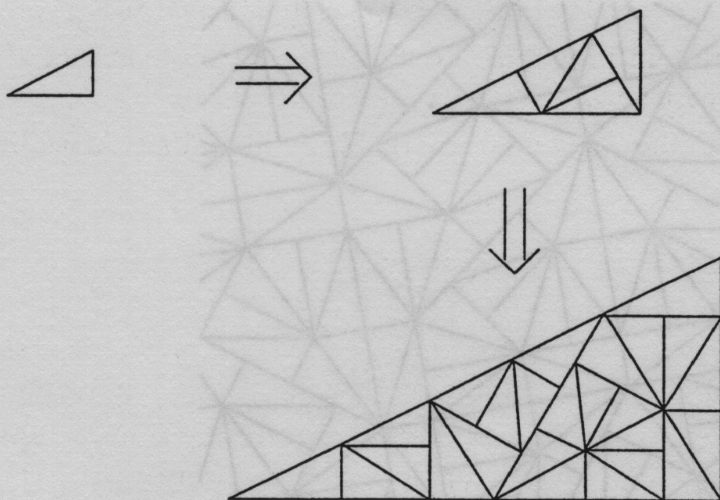
Fig. 1. Two iterations of the substitution rule.
