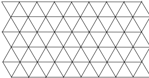
Figure 2. The triangular lattice.
