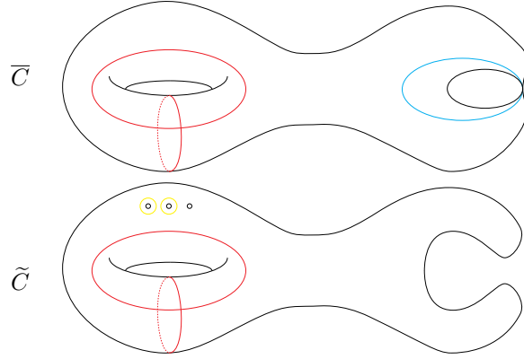
FIGURE 2. A compactification of our curve on top, and the normalization on the bottom.
