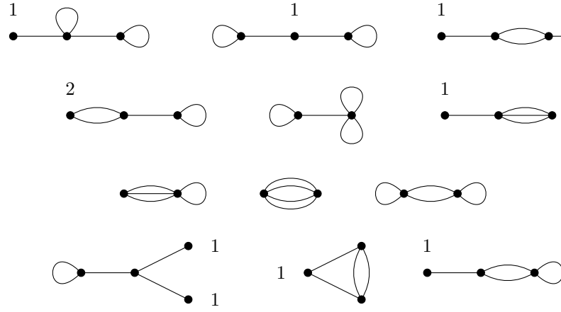
FIGURE 5. Stable graphs of genus 3 with 4 edges.
