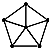
FIGURE 1. The graph W_5
